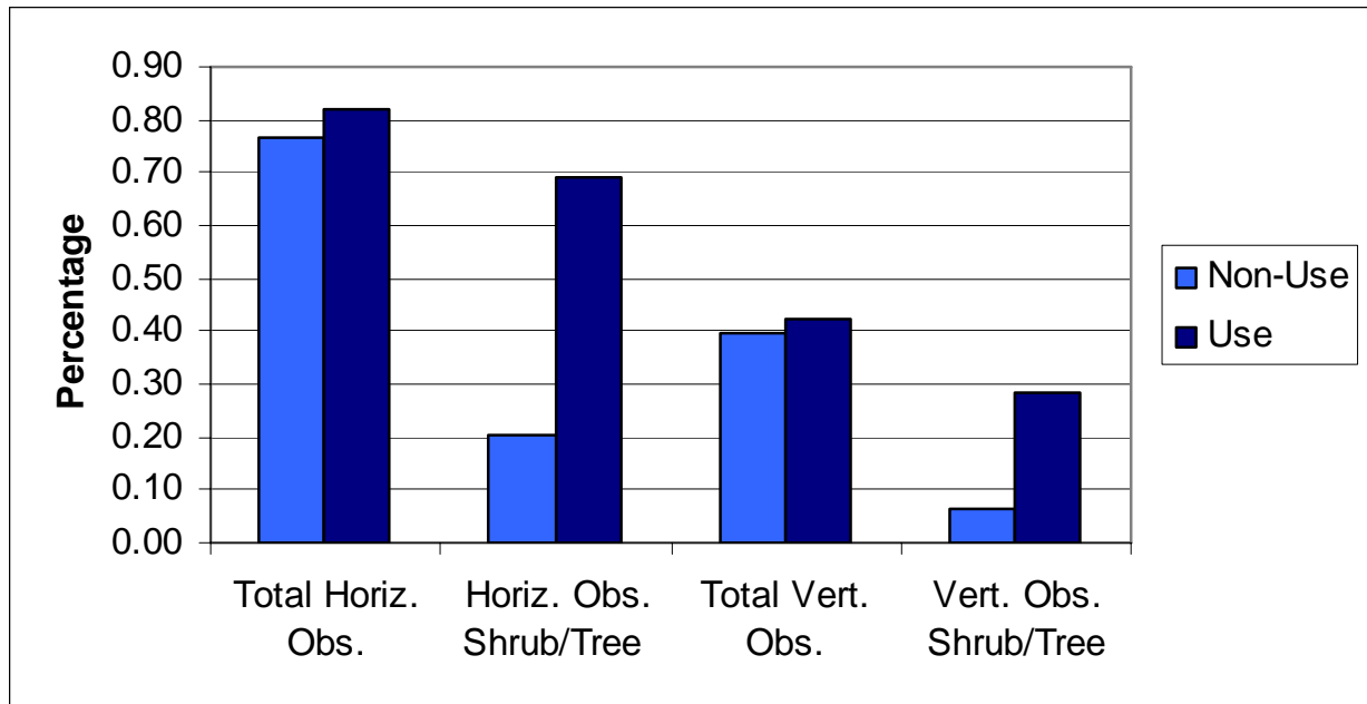
Figure 3. In comparisons of obscenity values at use and non-use sites—both shrub and tree only measures were significantly different ( P < 0.001 ), whereas total measures were not for horizontal (horiz.) and vertical (vert.) obscenity (obs.).
